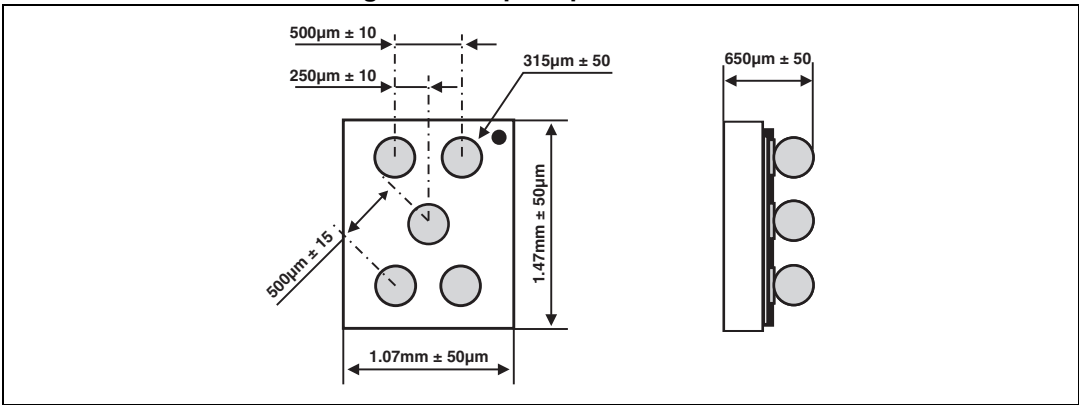
Figure 10. Flip Chip dimensions
