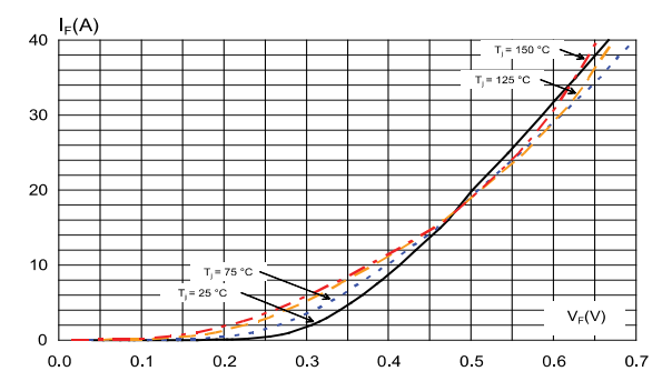
Figure 6: Forward voltage drop versus forward current (typical values)
