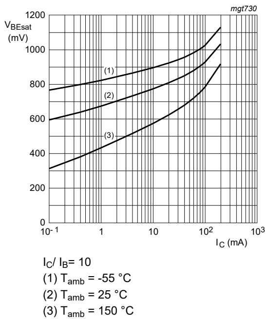
Fig. 11. BC847BQB: Base-emitter saturation voltage as a function of collector current; typical values
