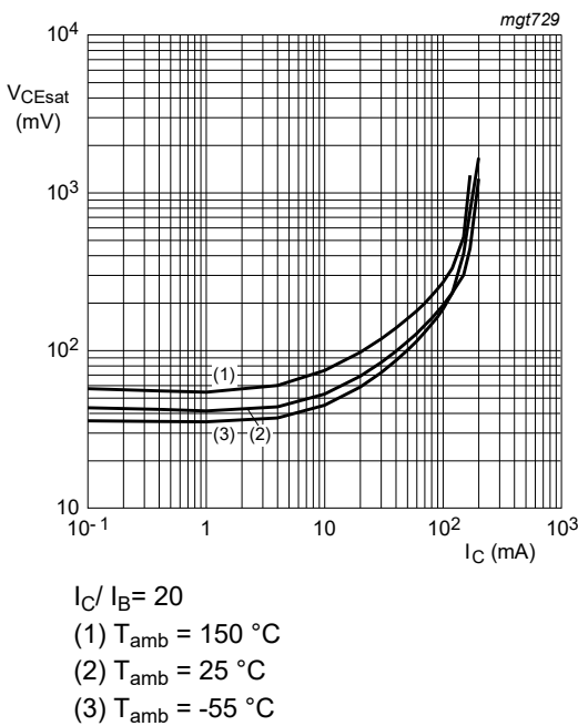
Fig. 10. BC847BQB: Collector-emitter saturation voltage as a function of collector current; typical values
