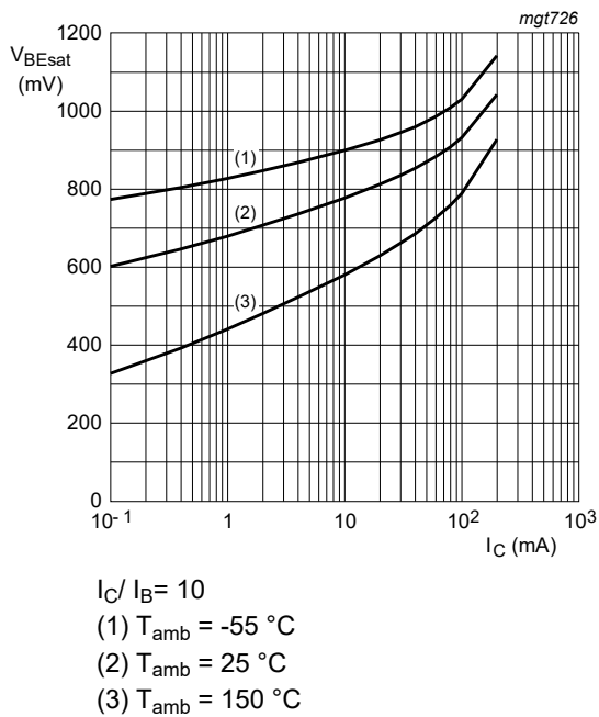
Fig. 7. BC847AQB: Base-emitter saturation voltage as a function of collector current; typical values
