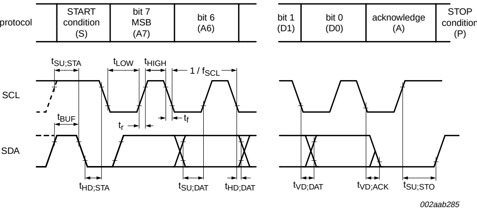
Fig 13. I 2 C-bus timing diagram
