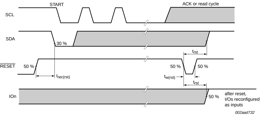
Fig 14. Definition of RESET timing
