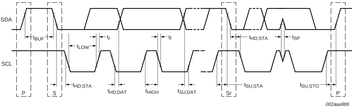
Fig 12. Definition of timing
