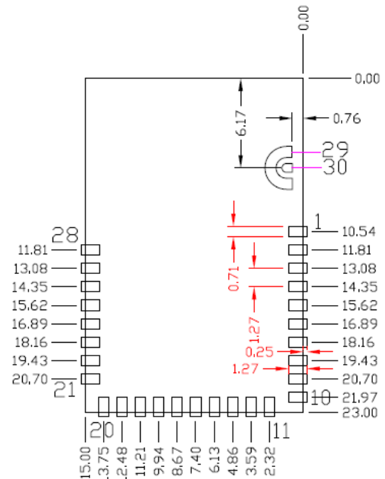
Top View (Seen on Host PCB)
