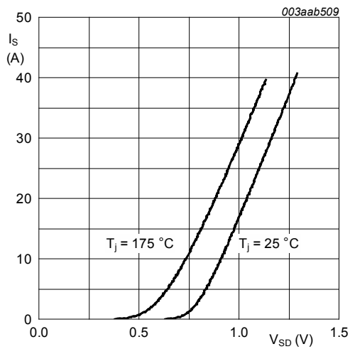
Fig. 7. Source current as a function of source-drain voltage; typical values
