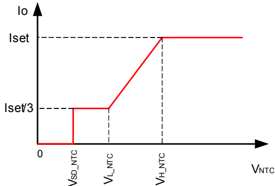
Figure 11: NTC Curve
