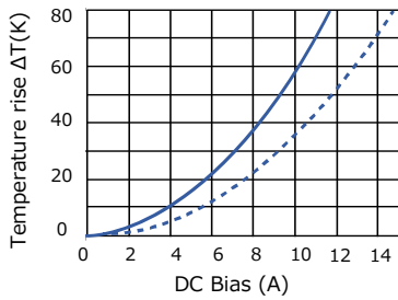
[ ETQP5M3R3YFM ]
