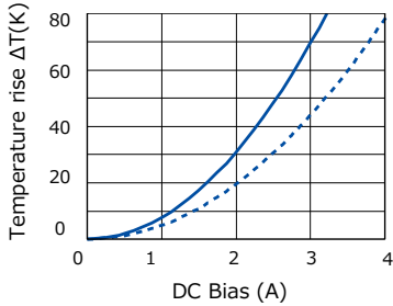
[ ETQP5M470YFM ]
