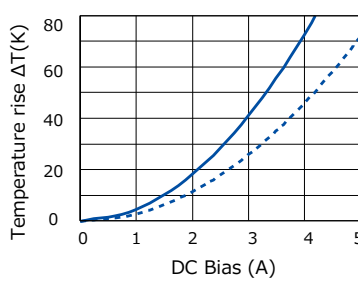
[ ETQP5M220YFM ]
