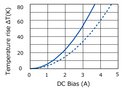
[ ETQP5M330YFM ]
