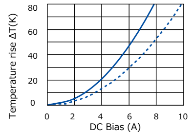
[ ETQP5M6R8YFM ]
