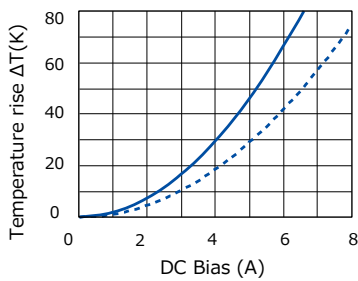
[ ETQP5M100YFM ]
