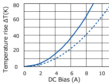
[ ETQP5M4R7YFM ]
