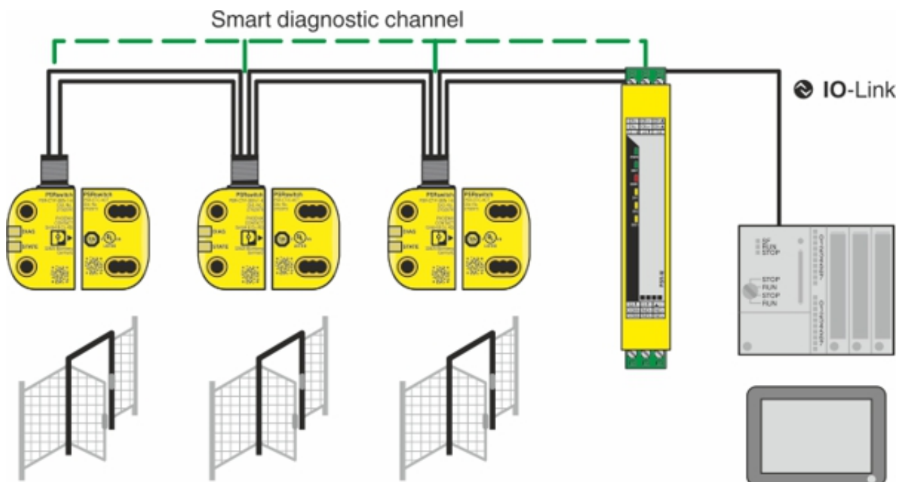
Application drawing
