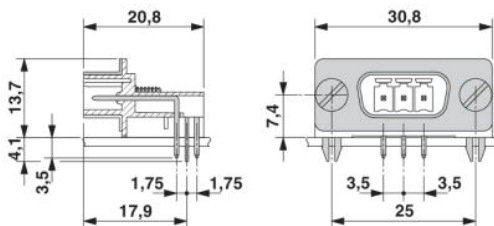
Dimensioned drawing
