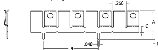
FIGURE 5 .25" Pin Spacing, No Standoff
