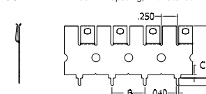
FIGURE 5 1.0" Pin Spacing, No Standoff, With Holes
