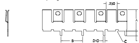
FIGURE 2 .50" Pin Spacing
