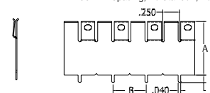
FIGURE 4 .50" Pin Spacing, With Standoff
