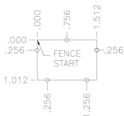
1.0" Pin Pattern
