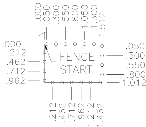
.25" Pin Pattern
