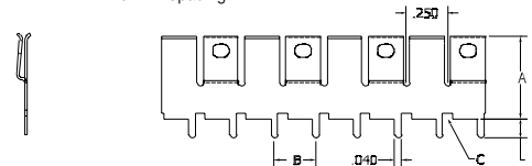
FIGURE 3 .25" Pin Spacing
