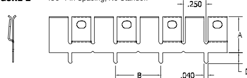
FIGURE 3 1.0" Pin Spacing, No Standoff
