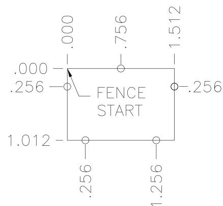
1.0" Pin Pattern
