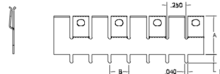
FIGURE 6 .25" Pin Spacing, No Standoff
