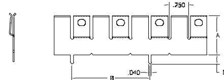
FIGURE 5 1.0" Pin Spacing, With Standoff
