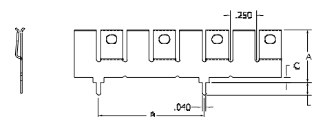
FIGURE 6 .25" Pin Spacing, No Standoff
