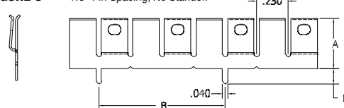
FIGURE 4 1.0" Pin Spacing, With Standoff
