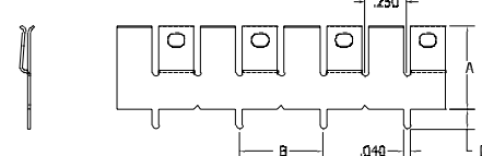
FIGURE 3 .50" Pin Spacing, With Standoff
