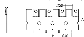
FIGURE 3 .50" Pin Spacing, No Standoff, No Holes
