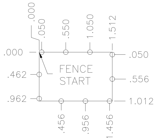
.50" Pin Pattern
