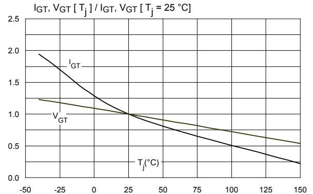
Figure 6. Relative variation of gate trigger current and gate voltage versus junction temperature (typical values)
