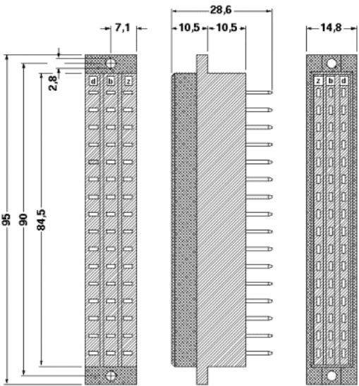
Dimensioned drawing
