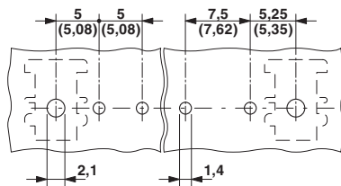
Vertically positioned header
