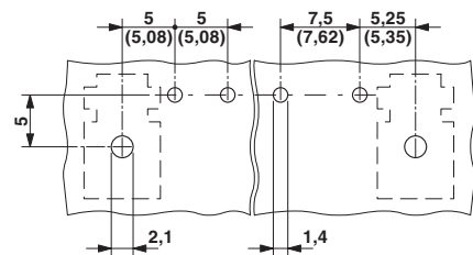
Horizontally positioned header
