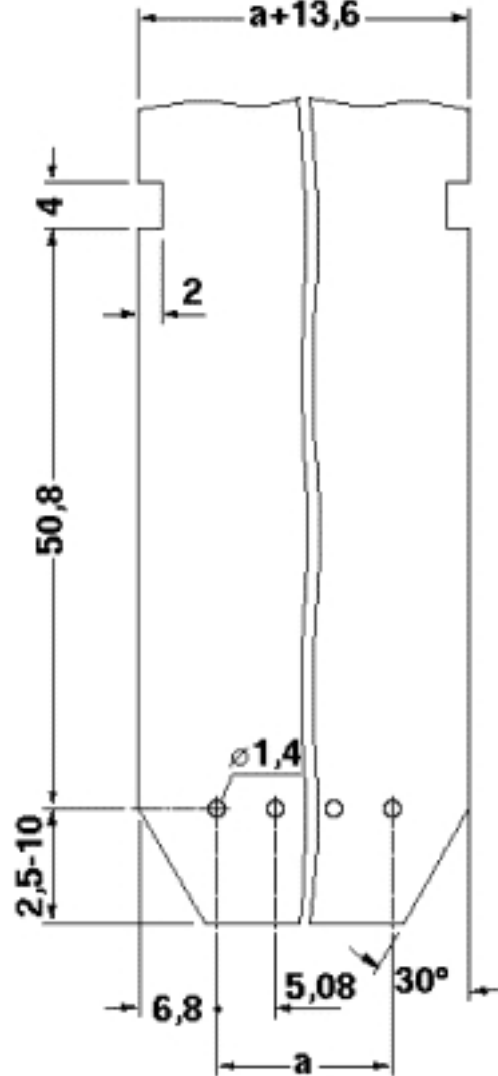
Drilling diagram
