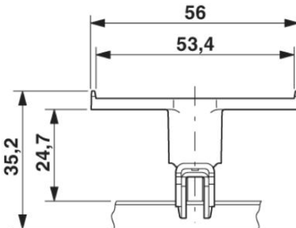
Dimensional drawing
