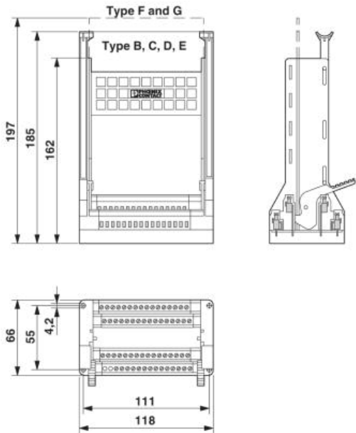
Dimensioned drawing
