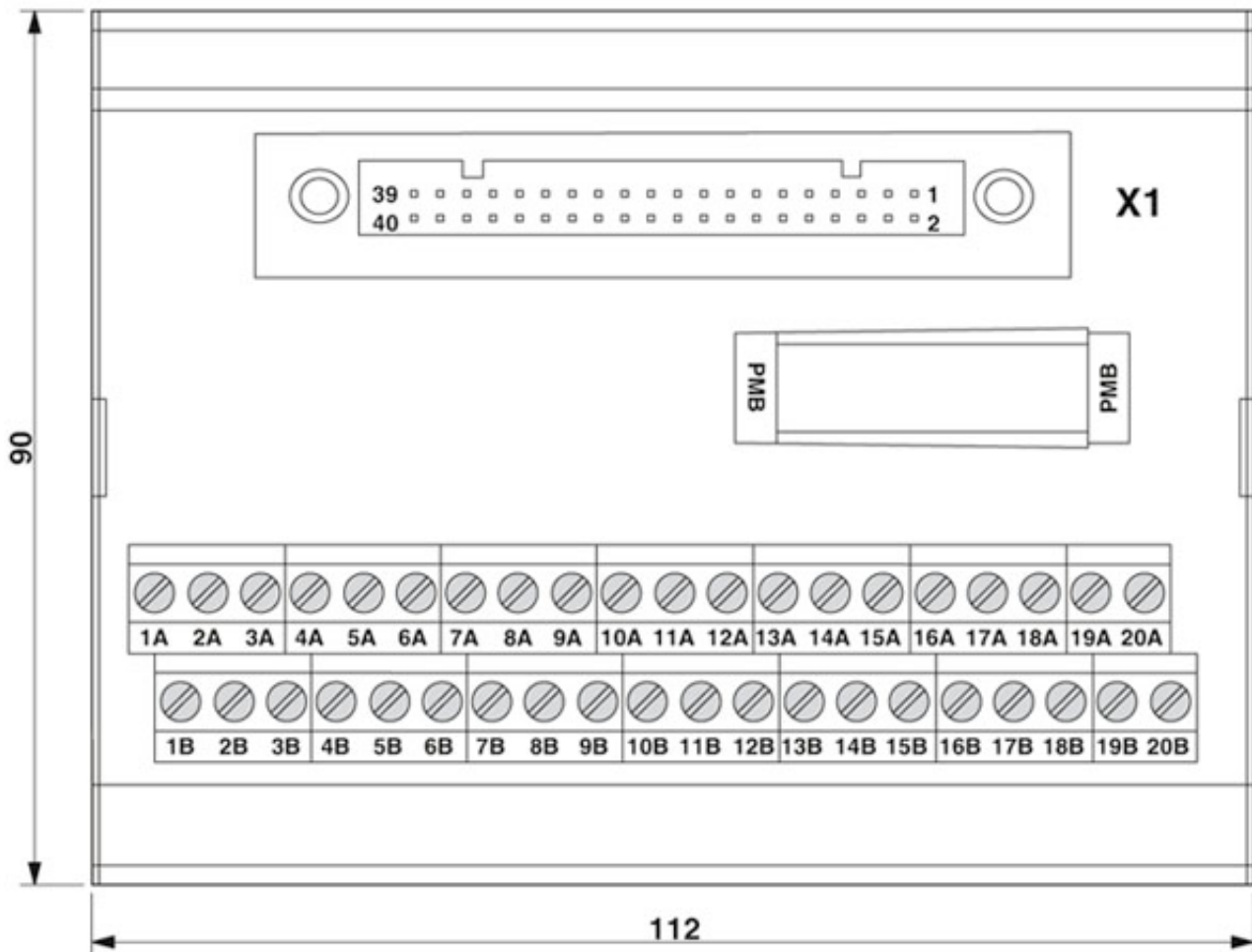
Dimensional drawing
