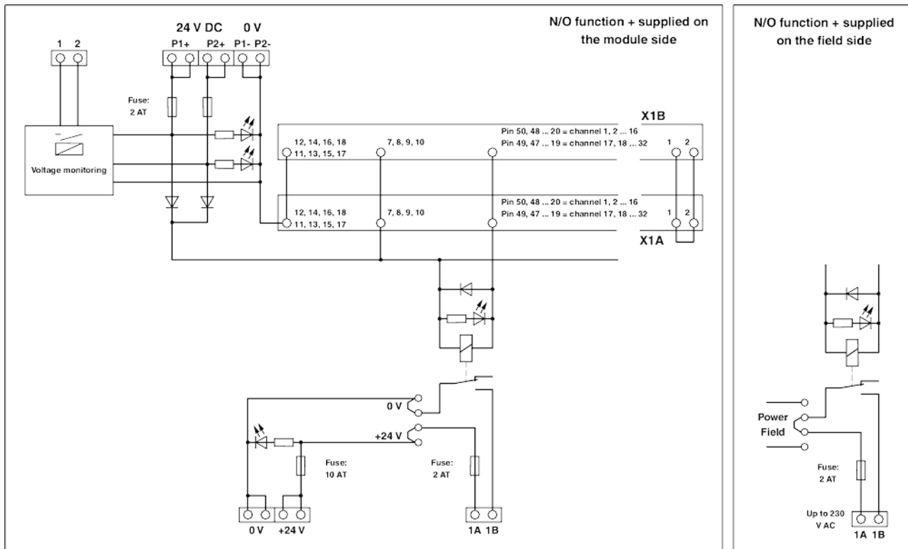
Circuit diagram
