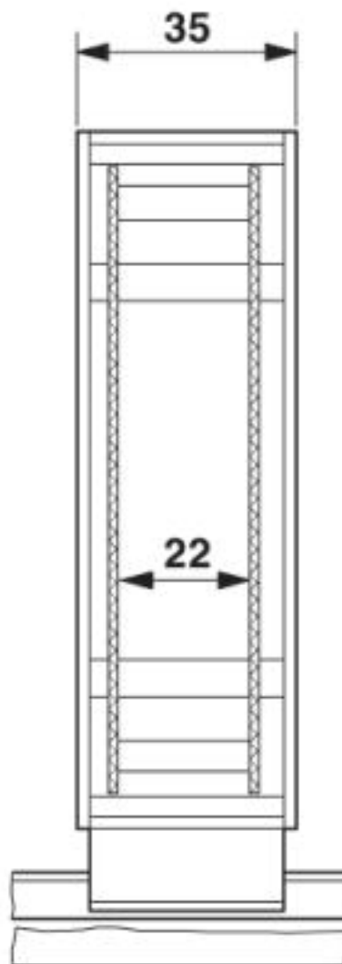
Maximum height of the components on the PCB with 2 PCBs
