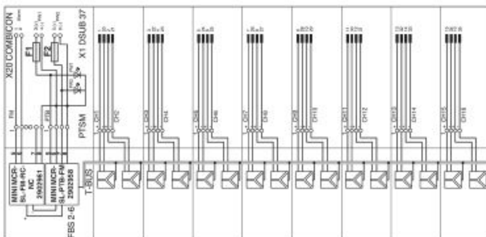
Circuit diagram
