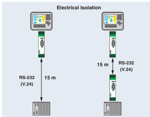
Electrical isolation
