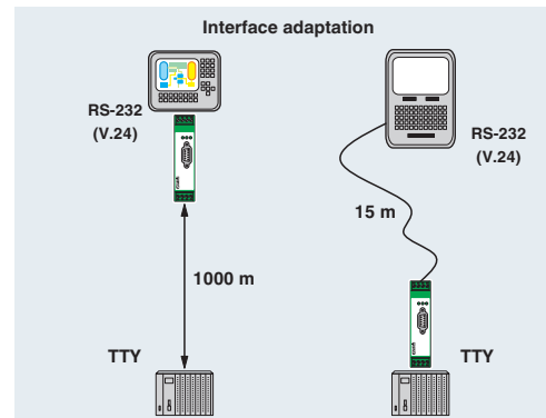
Interface adaptation
