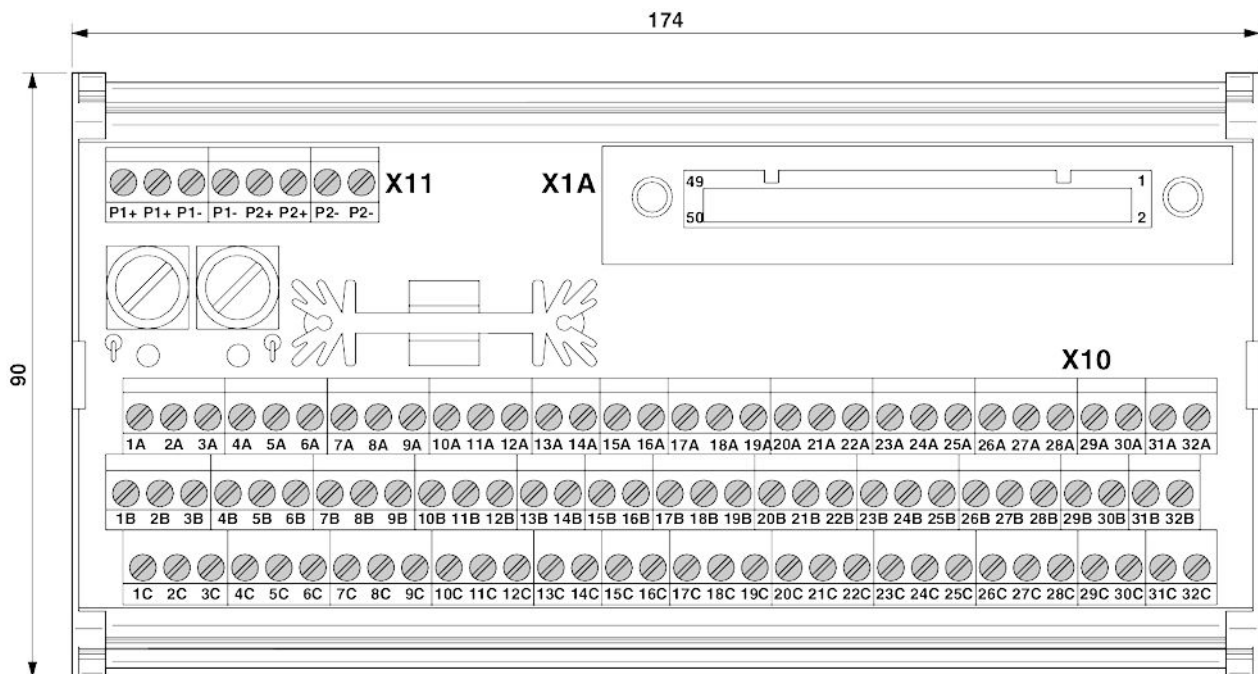
Dimensional drawing
