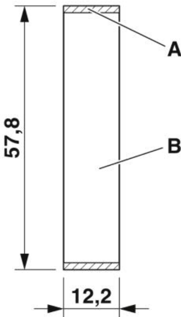
Dimensional drawing
