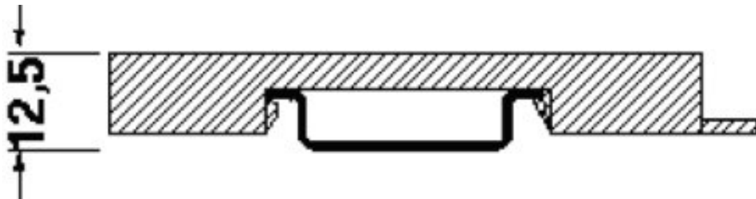
Dimensioned drawing
