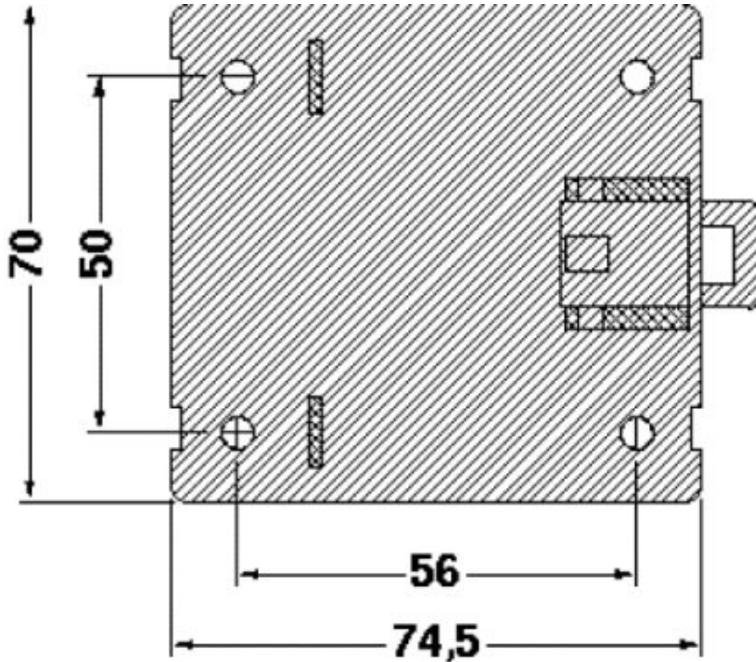
Dimensioned drawing
