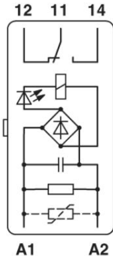
Circuit diagram
