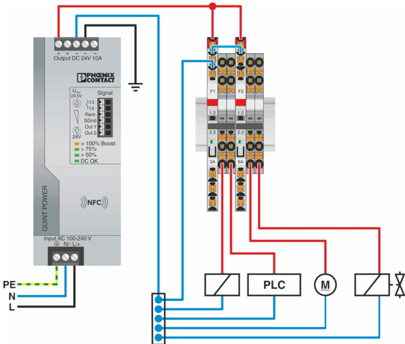
Application drawing
