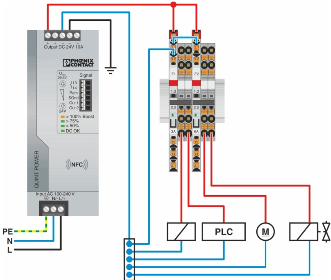
Application drawing
