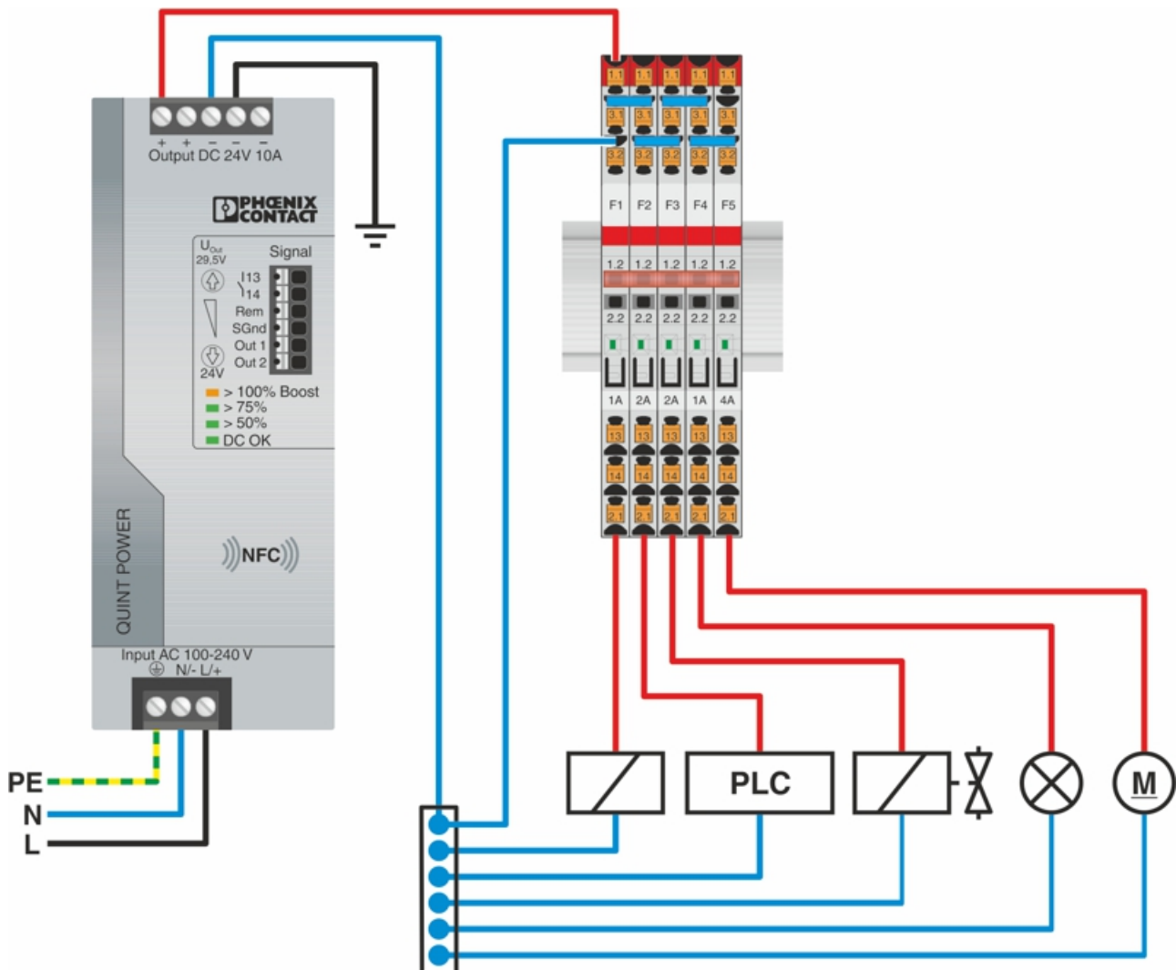
Application drawing
