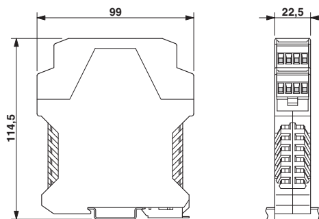
Dimensioned drawing
