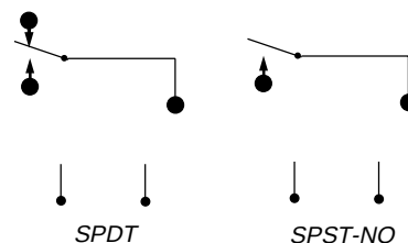
WIRING DIAGRAM BOTTOM VIEWS
