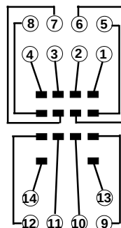
4PDT
