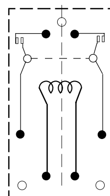
WIRING DIAGRAM
