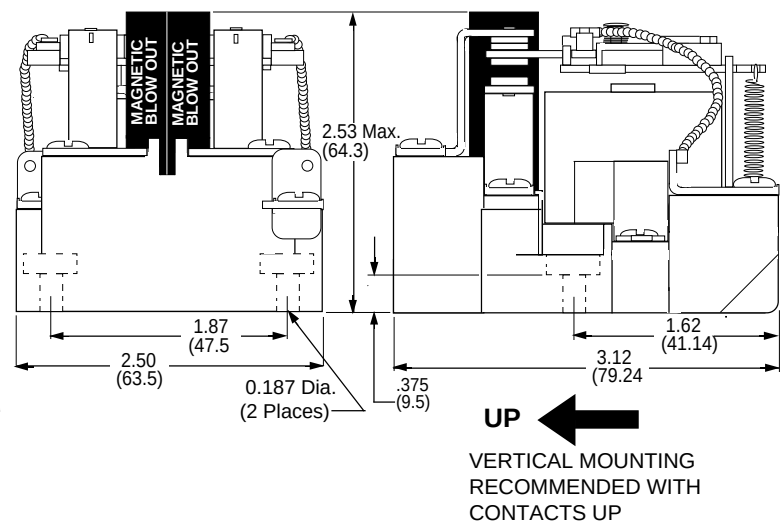
OUTLINE DIMENSIONS Dimensions shown in Inch & (Millimeters)
