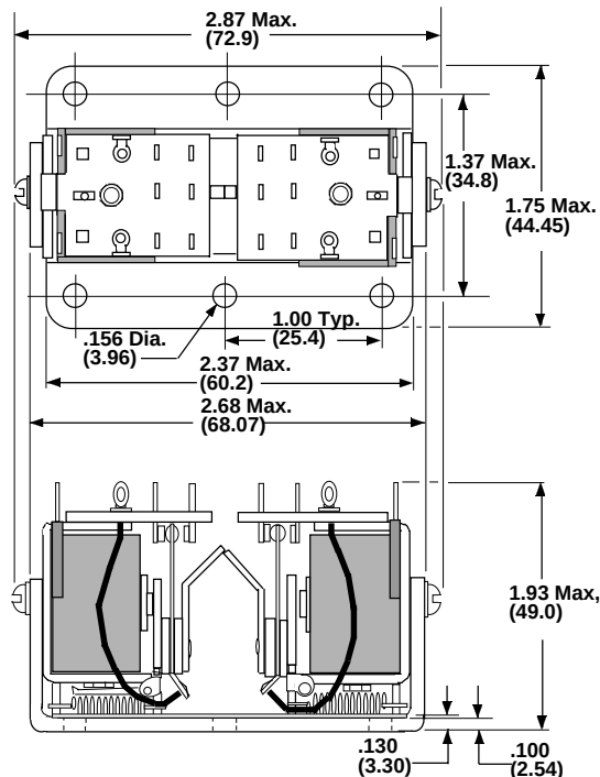
OUTLINE DIMENSIONS Dimensions shown Inchs & (Millimeters)
