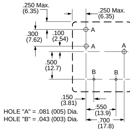
PC BOARD DRILL PATTERN BOTTOM VIEWS
