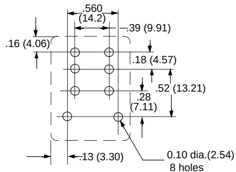
P.C. MOUNTING HOLE LAYOUT (BOTTOM VIEW)
