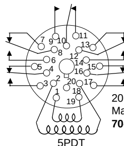
WIRING DIAGRAMS Shown from Pin End
