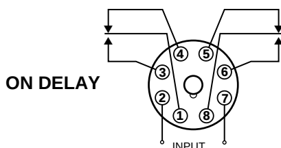
WIRING DIAGRAMS VIEWED FROM PIN END
