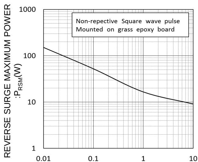
P_{RSM} - t CHARACTERISTICS
