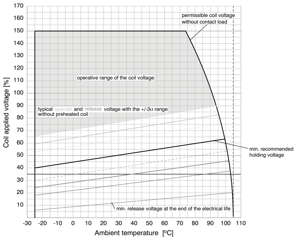
Coil voltage characteristics
