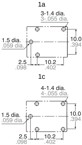
PC board pattern (Bottom view)
