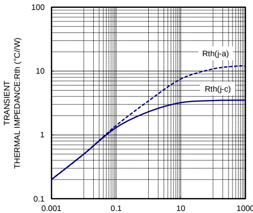
R_th-t CHARACTERISTICS
