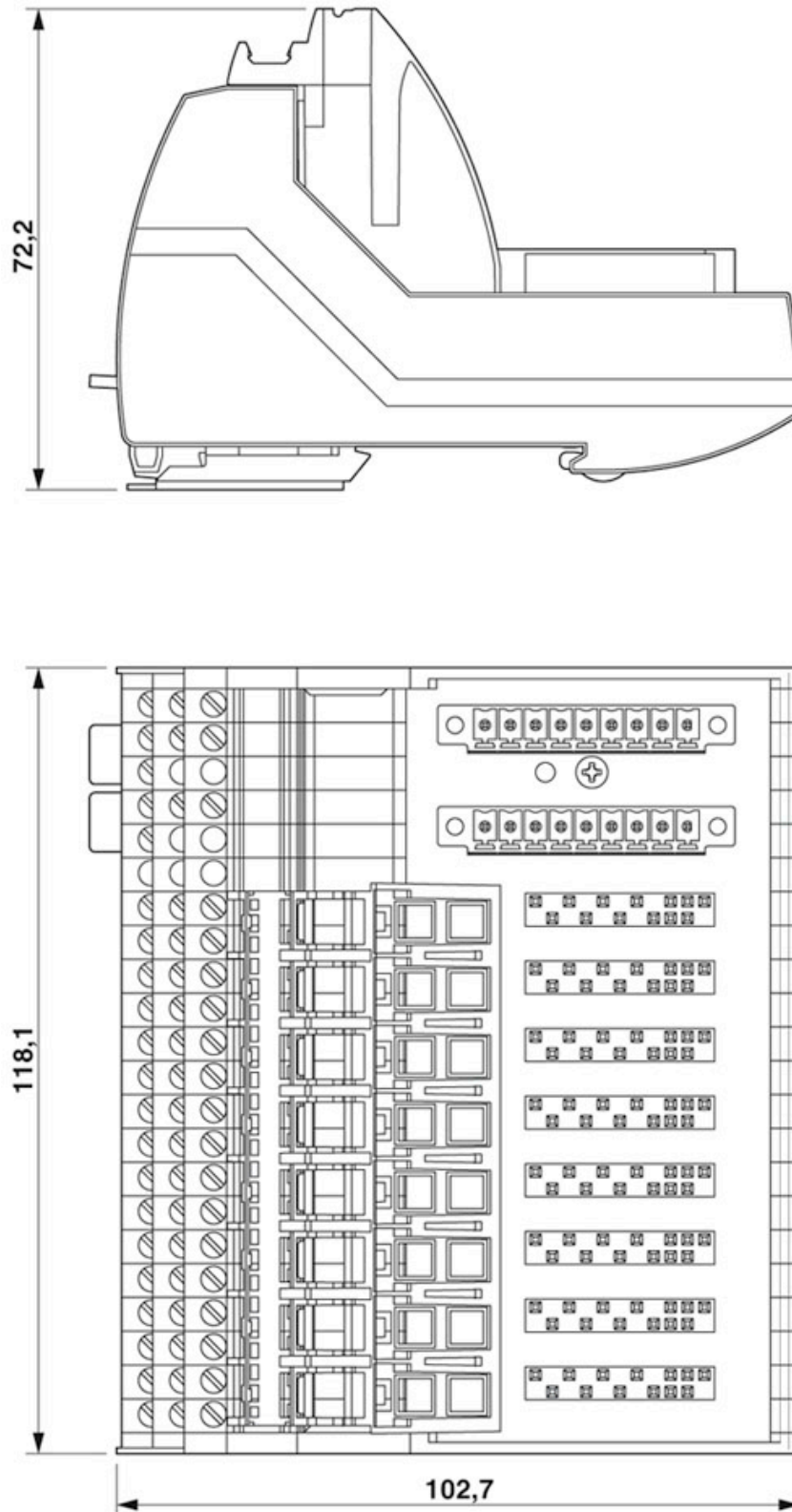
Dimensional drawing
