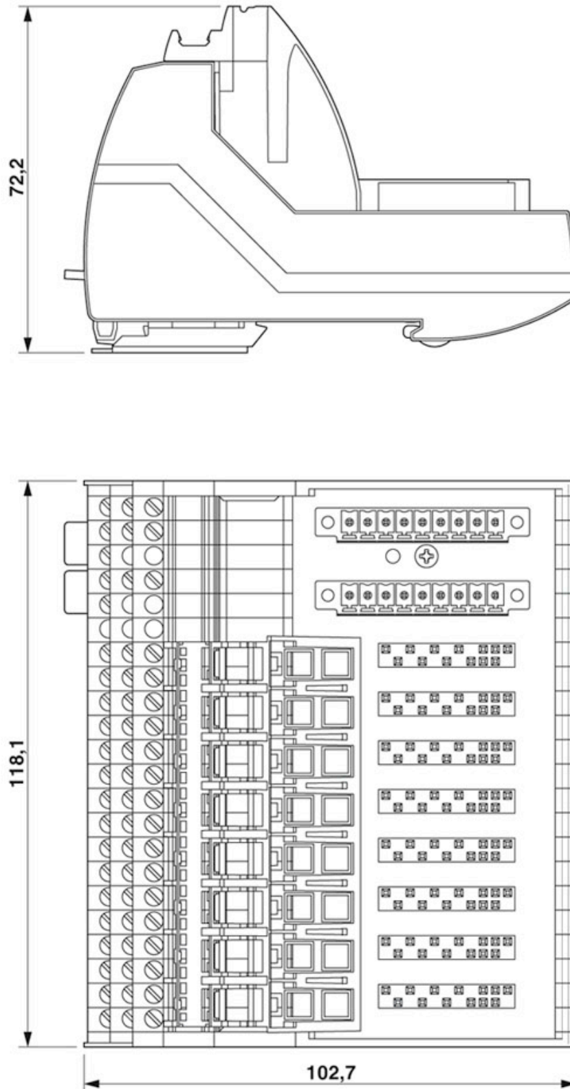
Dimensional drawing
