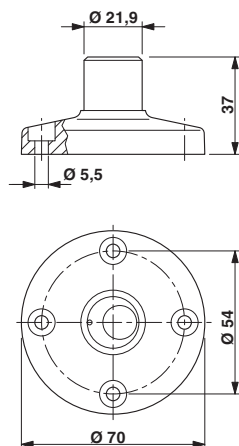
Dimensioned drawing
