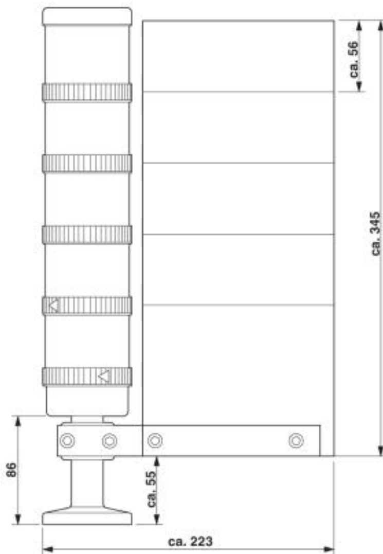
Dimensional drawing
