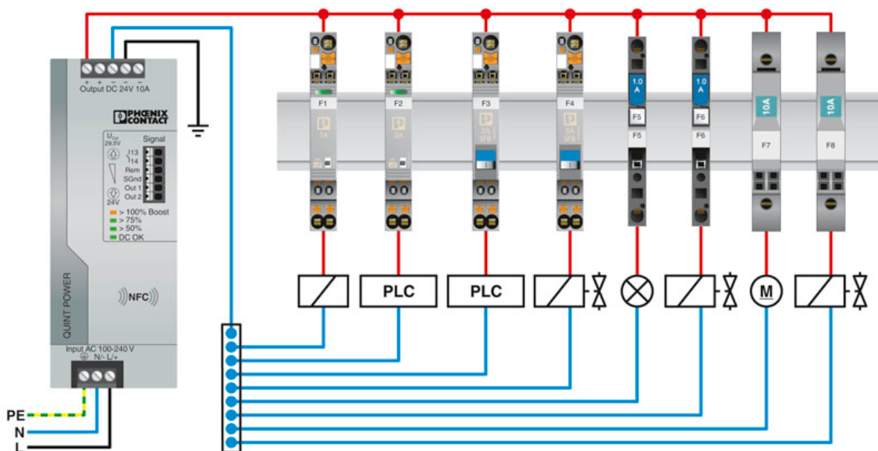
Application drawing
