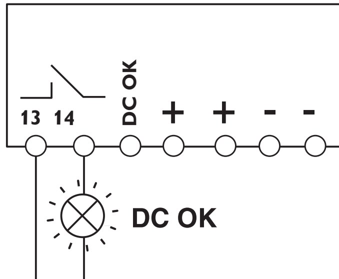
Circuit diagram
