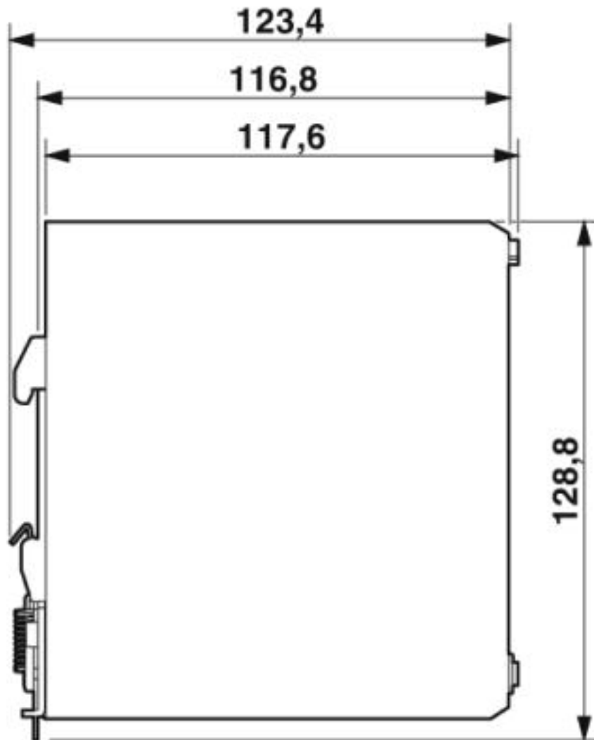
Dimensional drawing
