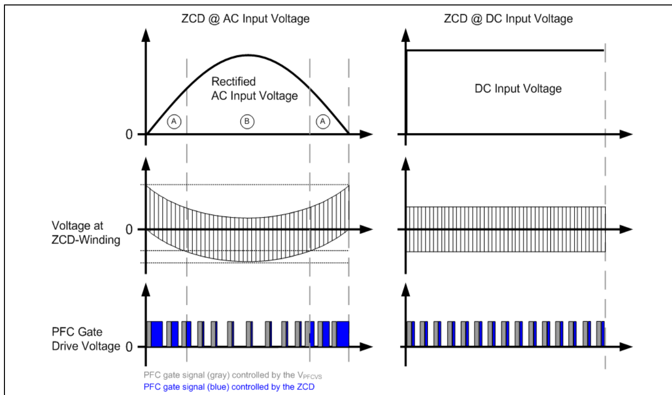
Figure 8 PFC THD Correction
