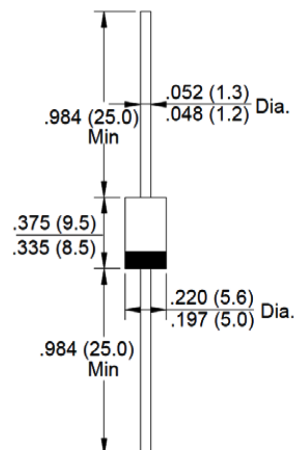
DO-201AA (DO-27)
