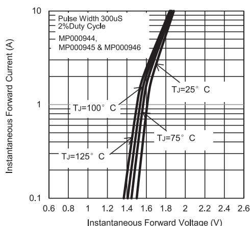
Fig. 6 - Typical Forward Characteristics
