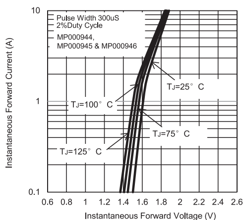
Fig. 6 - Typical Forward Characteristics
