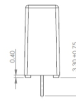
Mechanical Dimensions
