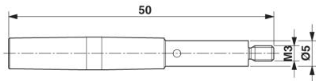
Dimensional drawing
