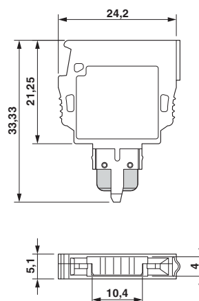
Dimensional drawing
