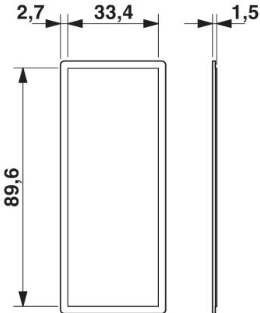
Dimensional drawing
