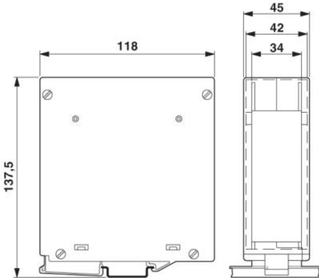
Dimensional drawing
