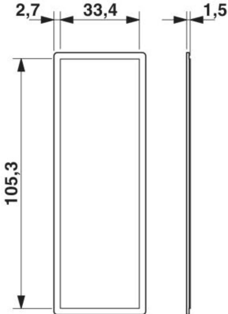
Dimensional drawing
