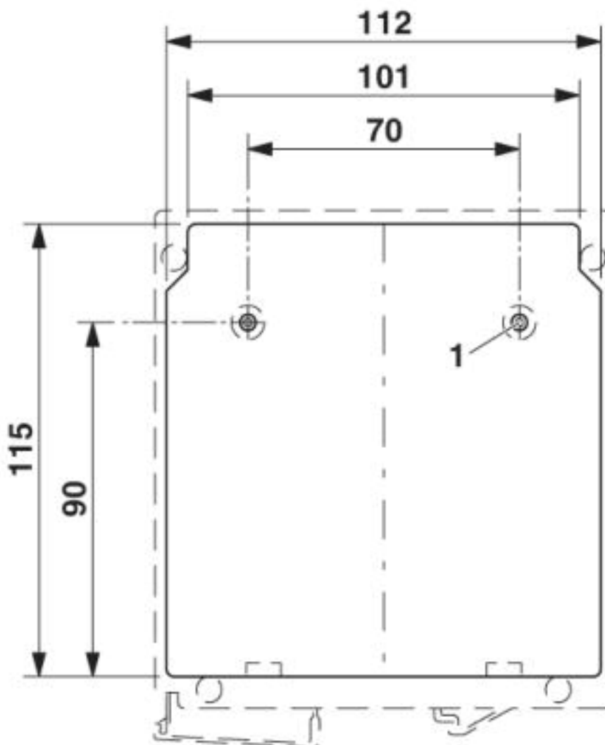
Dimensional drawing
