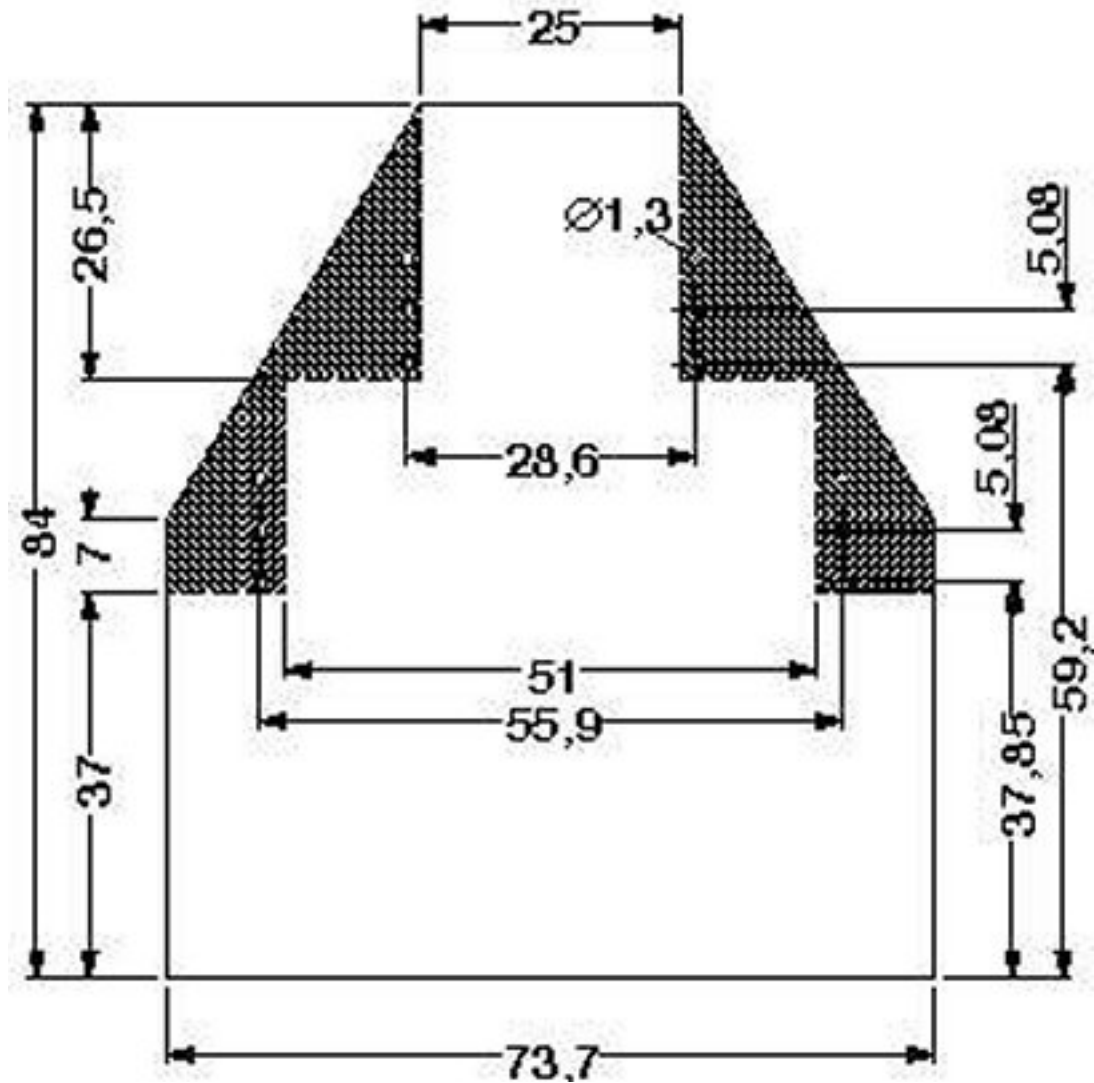
Dimensioned drawing
